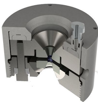
Diamond Anvil Cell
